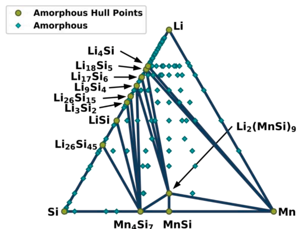
Fig. 6. Li-Mn-Si phase diagram showing the only system tending to extrude pure metal. Any Mn z Si (1-z) material will intersect the Mn-Li 4 Si phase equilibrium and displace Mn metal.
