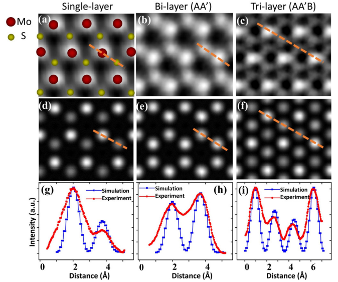
FIG. 3. Atomic-resolution ADF images of single-layer, bilayer (AA' stacking), and trilayer (AA'B stacking) CVD-grown MoS 2 in comparison with simulated images. (a)–(c) Experimentally observed atomic-resolution ADF images of single-layer, bilayer (AA' stacking), and trilayer (AA'B stacking) CVD-grown MoS 2 , respectively, after averaging the intensity of more than 10 unit cells from a larger area of the same stacking sequence. (d)–(f) Multislice simulation of ADF images of single-layer, bilayer (AA' stacking), and trilayer (AA'B stacking) MoS 2 with the same beam energy, convergence angle, and collection angles for the experiment. (g)–(i) Line scans across lattice points indicated by the orange lines in (a)–(c) and (d)–(f), showing the comparison of intensity of these lattice points in simulated and experimental ADF images for single-layer, bilayer (AA' stacking), and trilayer (AA'B stacking) CVD-grown MoS 2 , respectively.
