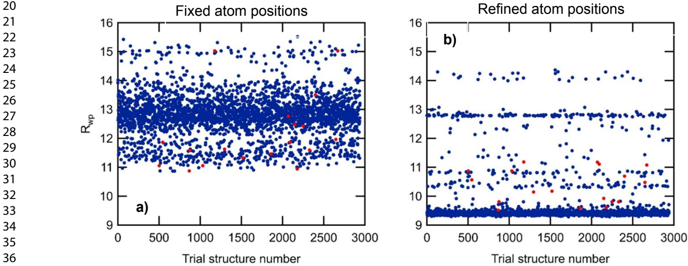
Figure 5. Comparison of R_{wp} values for all 2,940 trial structures obtained after Rietveld refinements in which atom positions were fixed (left) or were freely refined, allowing structures to be optimized (right). Refinements in centered space groups are indicated with red symbols, and are shown in more detail in Figure S1, while R_{wp} histograms are shown in Figure S2.
