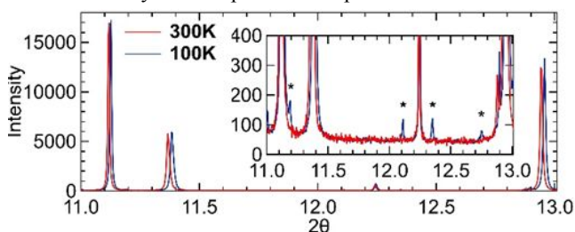
Figure 2. Comparison of synchrotron XRD data ( \lambda = 0.62 Å) collected on NVPF at 300 K (RT, red) and 100 K (LT, blue). Inset is shown at an approximately 50X zoom, highlighting additional low-intensity supercell peaks associated with Na cation ordering (*).
