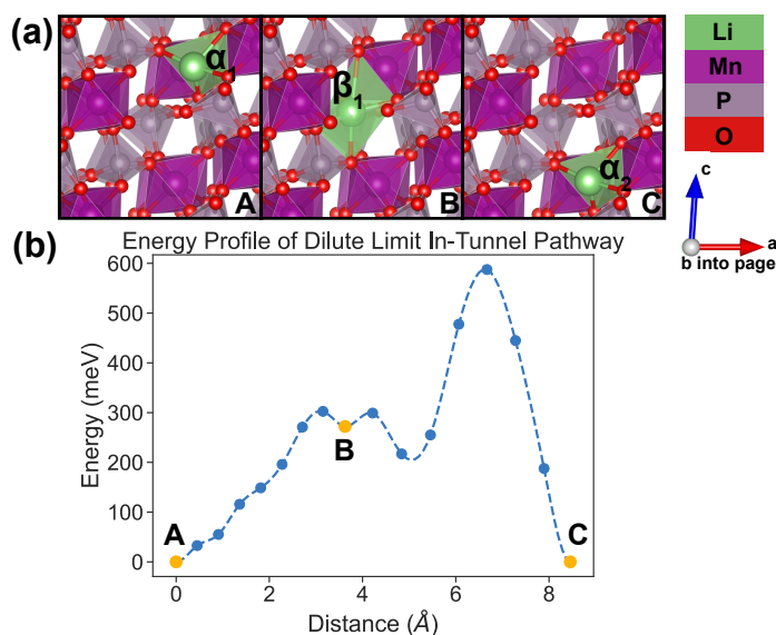
Fig. 6 Li-ion evolution of the along-tunnel pathway ( Pathway I ) in the dilute limit. (a) shows images along the pathway, and Li positions labeled \alpha_1 , \beta_1 and \alpha_2 have the same positions with identical labels in FIG. 4. (b) shows calculated energy evolution as a function of Li migration distance, where labels \alpha_1 , \beta_1 and \alpha_2 correspond to the images in (a).
