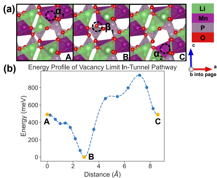
Fig. 8 Li vacancy evolution of the along-tunnel pathway ( Pathway I ) in the vacancy limit. (a) shows images along the pathway, where dashed circles indicate positions of vacancies; vacancy positions labeled \alpha_1 , \beta_1 and \alpha_2 have the same positions with identical labels in FIG. 4. (b) shows calculated energy evolution as a function of vacancy migration distance, where labels \alpha_1 , \beta_1 and \alpha_2 correspond to the images in (a).
