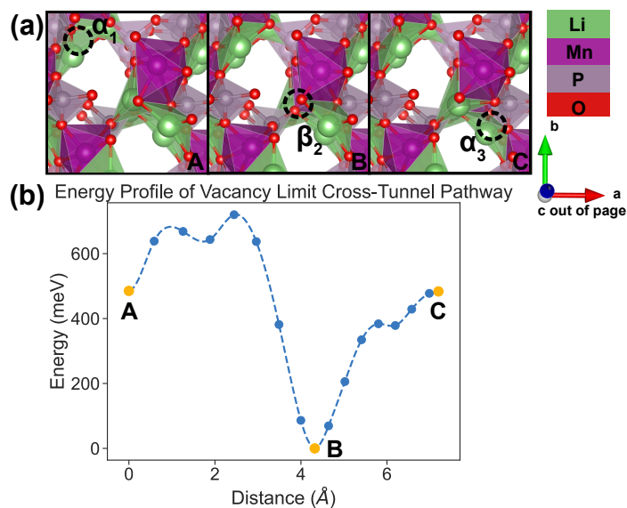
Fig. 9 Li vacancy evolution of the cross-tunnel pathway ( Pathway II ) in the vacancy limit. (a) shows images along the pathway, where dashed circles indicate positions of vacancies; vacancy positions labeled \alpha_1 , \beta_2 and \alpha_3 have the same positions with identical labels in FIG. 4. (b) shows calculated energy evolution as a function of vacancy migration distance, where labels \alpha_1 , \beta_2 and \alpha_3 correspond to the images in (a).
