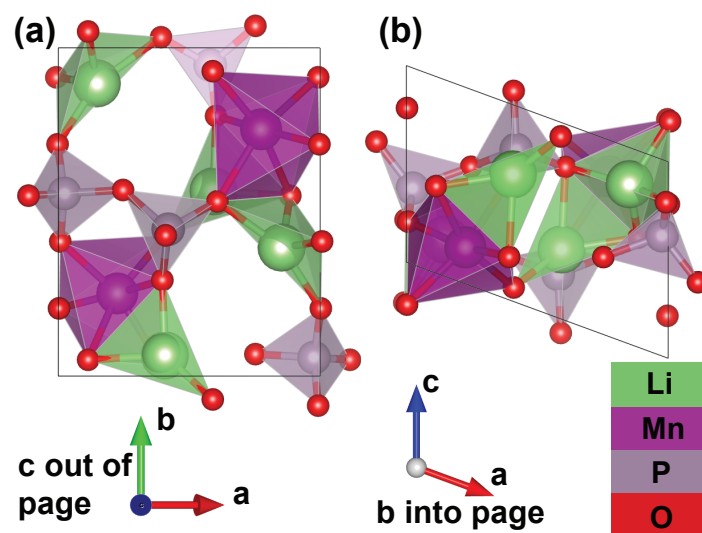
Fig. 3 The unit cell structure of the fully discharged \gamma - Li_2MnP_2O_7 . (a) shows the c -axis, the tunnel direction, pointing into and out of page, and (b) shows the c -axis pointing up and down. This structure is in the P2_1 spacegroup ( a=7.27\text{\AA} , b=8.55\text{\AA} , c=5.12\text{\AA} , and \alpha=90^\circ , \beta=110^\circ , \gamma=90^\circ ). Identifier from the Materials Project: mp-770967.
