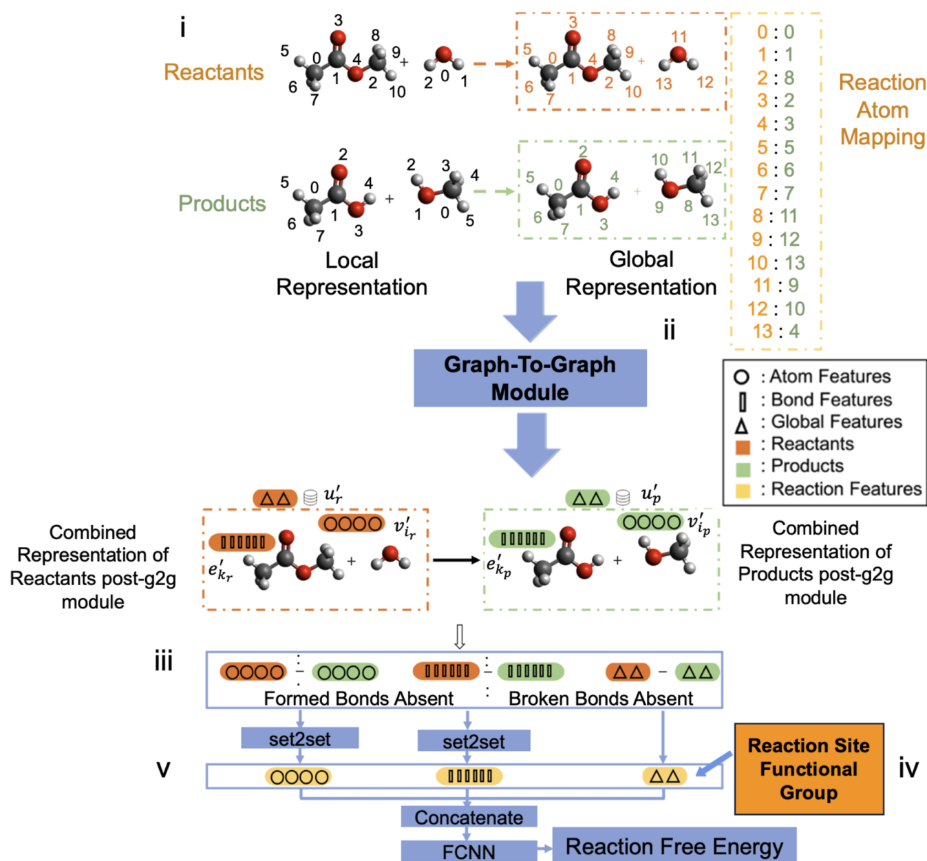
Figure 2. GNN Architecture: The user inputs atom-mapped sets of reactants and products (i) which undergo message-passing and update steps (ii). Using the user-specified mappings, these updated features are mapped to a global reaction graph (iii) where functional groups are the reaction site is added as a global feature (iv). Embeddings of bond and atom features plus global features directly serve as the fixed-size vector used in a conventional dense neural network for property prediction.
