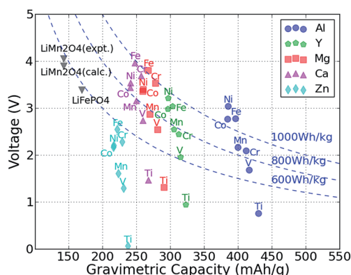
Fig. 2 The computed average voltage vs. gravimetric capacity for intercalation of A = Zn, Ca, Mg, Y and Al in various M_2O_4 spinels up to composition AM_2O_4 . The redox-active metal is marked next to each point. Dashed curves show the specific energy of 600 \text{ Wh kg}^{-1} , 800 \text{ Wh kg}^{-1} and 1000 \text{ Wh kg}^{-1} , respectively. The spinel LiMn_2O_4 and olivine LiFePO_4 data points are also marked on the plot for comparison. 22,36,43
