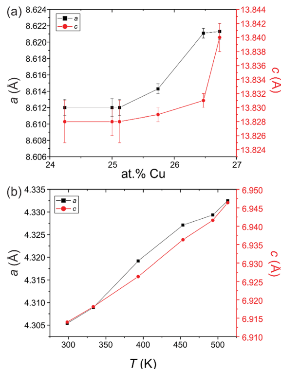
Fig. 7 (a) The room-temperature lattice parameters for \text{YCu}_x\text{Te}_2 samples with different nominal Cu content. (b) The temperature dependence of the lattice parameters for \text{YCu}_{1.04}\text{Te}_2 , where the lattice parameters were refined for the small cell (the standard deviations are smaller than the size of the symbols used).
