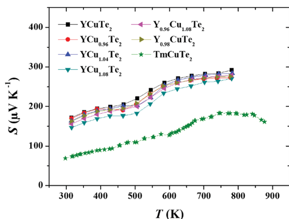
Fig. 10 The Seebeck coefficient increases with temperature for the parent \text{YCuTe}_2 compound and intrinsically doped samples. All investigated samples have higher Seebeck coefficient than that of \text{TmCuTe}_2 .
