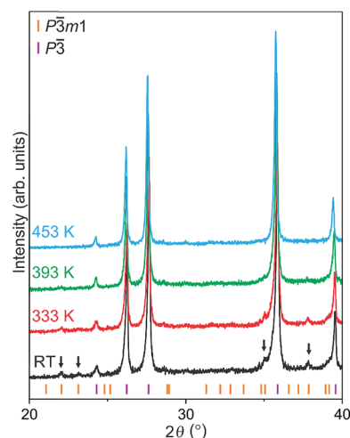
Fig. 5 HT-XRD patterns of YCu 1.04 Te 2 sample. The intensity of the main supercell reflections indicated by arrows decreases with increasing temperature and vanishes completely at 453 \text{ K} , i.e. above the phase transformation.
