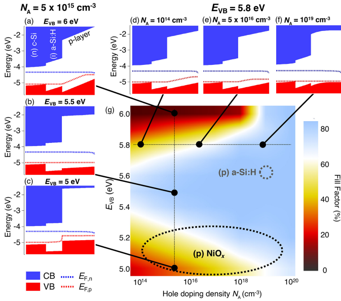
Fig. 4. Band diagrams at maximum power point (MPP) for six different p-layer combinations of VB edge energy ( E_{VB} ) and hole doping density ( N_A ). (a)–(c) The three diagrams on the left are at constant N_A and varied E_{VB} , while (d)–(f) the three upper diagrams are at constant E_{VB} and varied N_A . As described in the legend (lower left corner), blue shadings are the conduction band states in the device (CB), dotted blue lines are the electron QFLs ( E_{F,n} ), red shadings are the valence band states in the device (VB), and dotted red lines are the hole QFLs ( E_{F,p} ). Black circles indicate the location of each condition studied on (g), the FF heat map from Fig. 3(c). For reference, the approximate range of E_{VB} and N_A reported experimentally are plotted in (g) for p-type \text{NiO}_x and p-type a-Si:H with dotted ovals.
