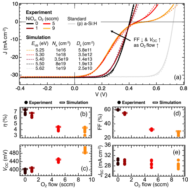
Fig. 6. (a) JV curves for \text{NiO}_x -contacted SHJ solar cells (solid lines), with oxygen flow rates in the \text{NiO}_x layer of 0, 1, 5, and 9 sccm, and for a standard cell with a (p) a-Si:H contact. Fits for the simulations used in this study are shown with dashed lines, with simulated parameters reported in the legend. Statistical analysis of these cells for solar cell performance parameters: (b) efficiency ( \eta ), (c) V_{\text{OC}} , (d) fill factor (FF), and (e) J_{\text{SC}} .
